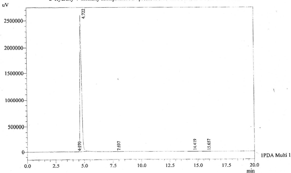
Chromatogram 2'-Hydroxy-4'-methoxy acetophenone D:\pmonence\Data\2013\SEPT-2013\300913J.lcd
